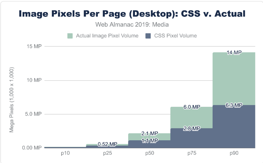
Figure 4.4. Image pixels per page (desktop): CSS versus actual.
