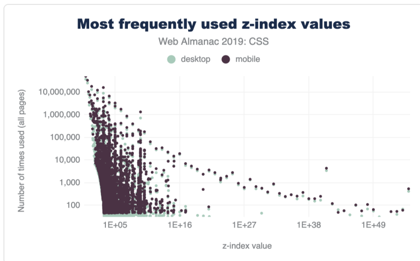
Figure 2.21. Most frequently used z-index values.
