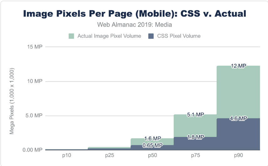
Figure 4.3. Image pixels per page (mobile): CSS versus actual.
