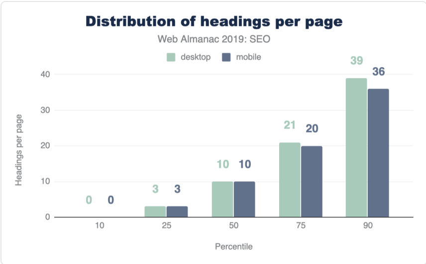
Figure 10.2. Distribution of the number of headings per page.
