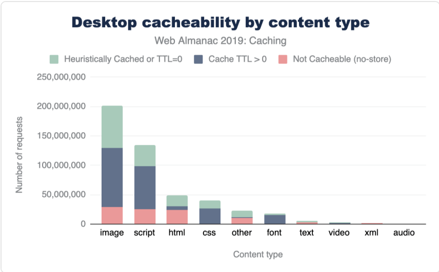
Figure 16.5. Distribution of cacheability by content type for desktop.
