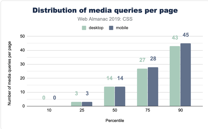
Figure 2.27. Distribution of the number of media queries per page.
