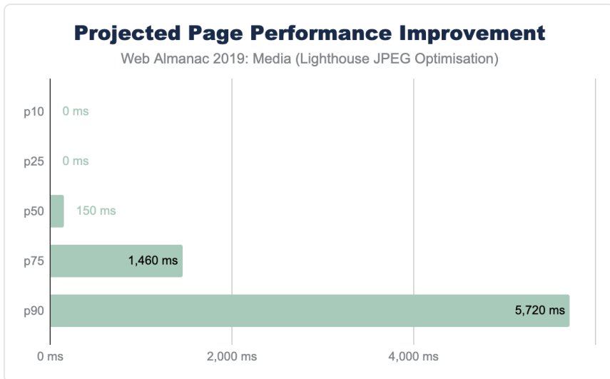
Figure 4.13. Projected page performance improvements from image optimization from Lighthouse.
