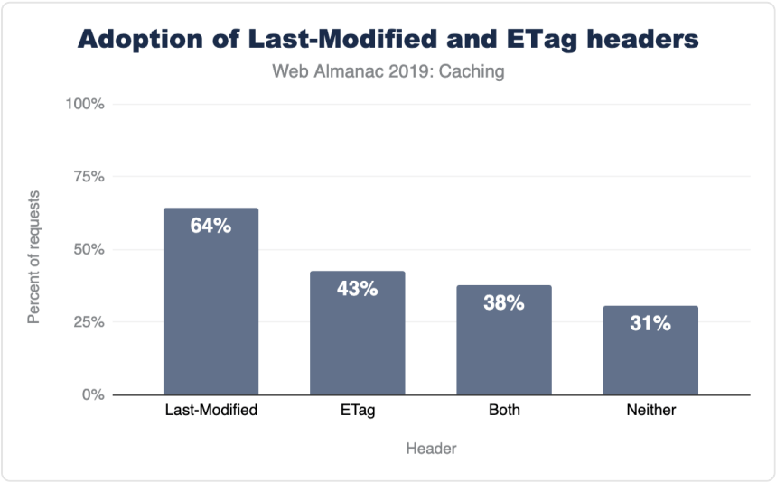
Figure 16.12. Adoption of validating freshness via Last-Modified and ETag headers for desktop websites.
