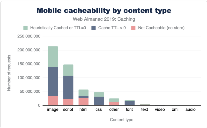
Figure 16.6. Distribution of cacheability by content type for mobile.
