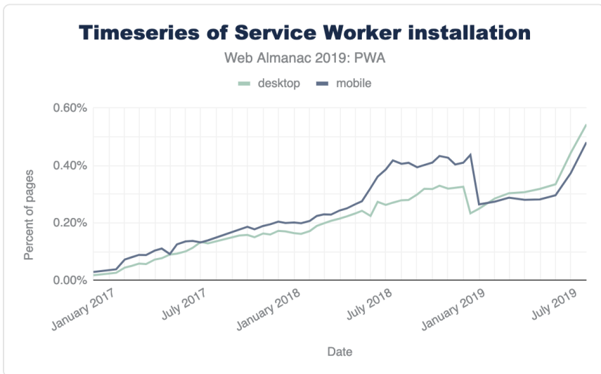
Figure 11.2. Service Worker installation over time for desktop and mobile.
