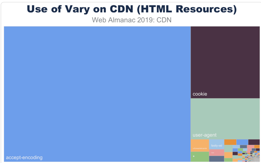
Figure 17.24. Usage of Vary for HTML served from CDNs.
