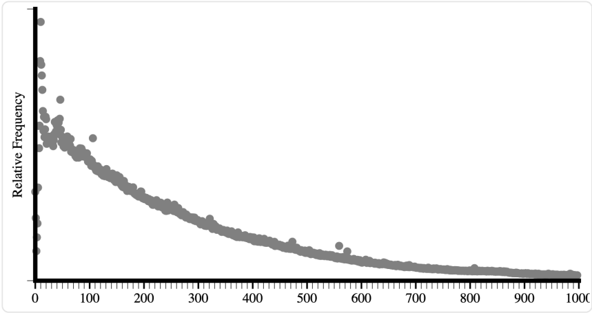
Figure 3.2. Distribution of Hixie’s 2005 analysis of element frequencies.
