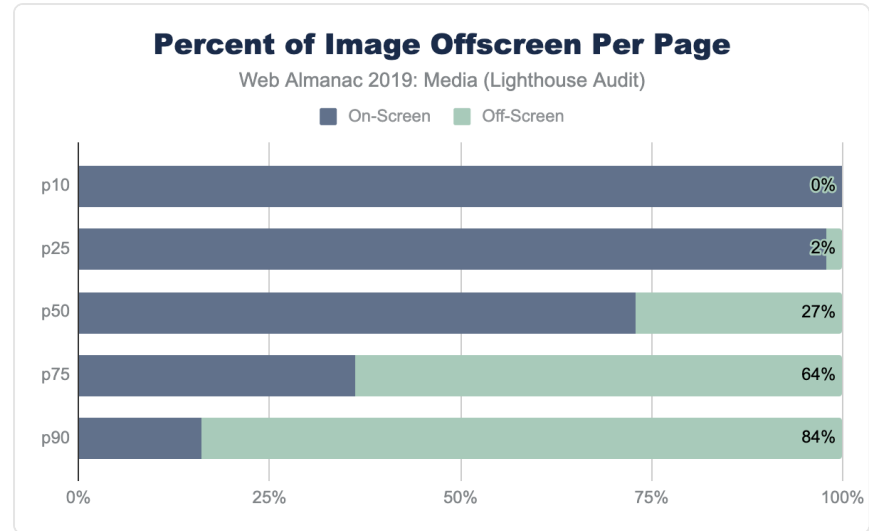
Figure 4.19. Lighthouse audit: Offscreen.
