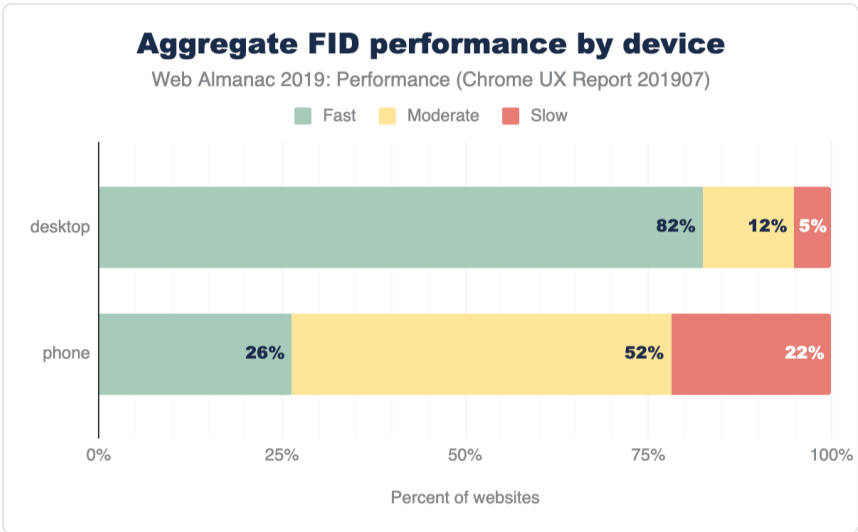
Figure 7.16. Distribution of websites labeled as having fast, moderate, or slow FID, broken down by device type.
