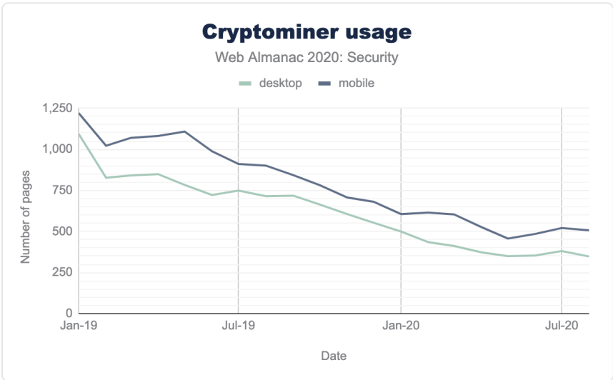
Figure 11.33. Cryptominer usage.
