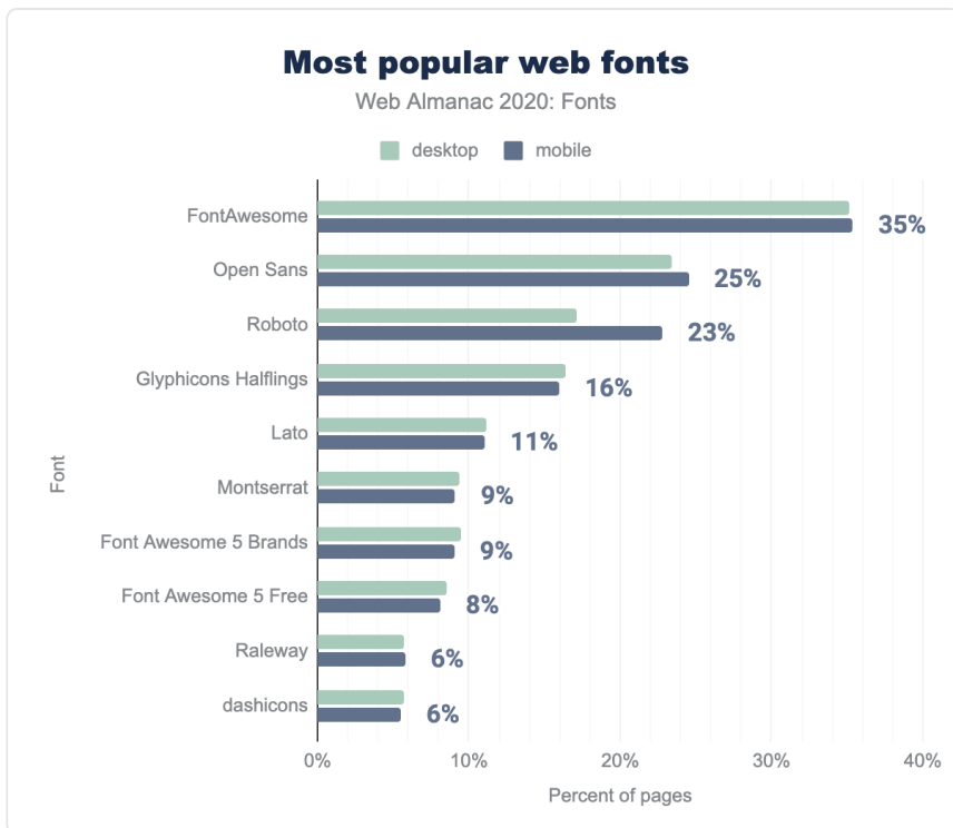
Figure 4.17. Popular typefaces.
