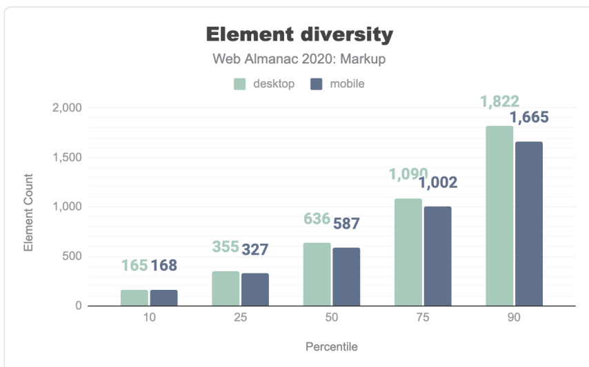
Figure 3.7. Distribution of the total number elements per page by percentile.
