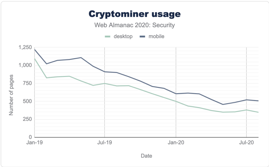
Figure 11.33. Cryptominer usage.
