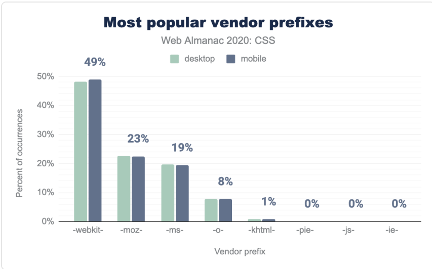
Figure 1.55. Relative popularity of vendor prefixes, as a percent of occurrences.
